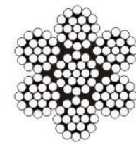
6×19+WSC
