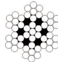
6×7+WSC
