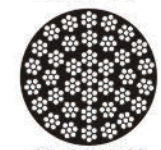
36×7+WSC
