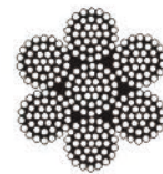
6×37+WSC
